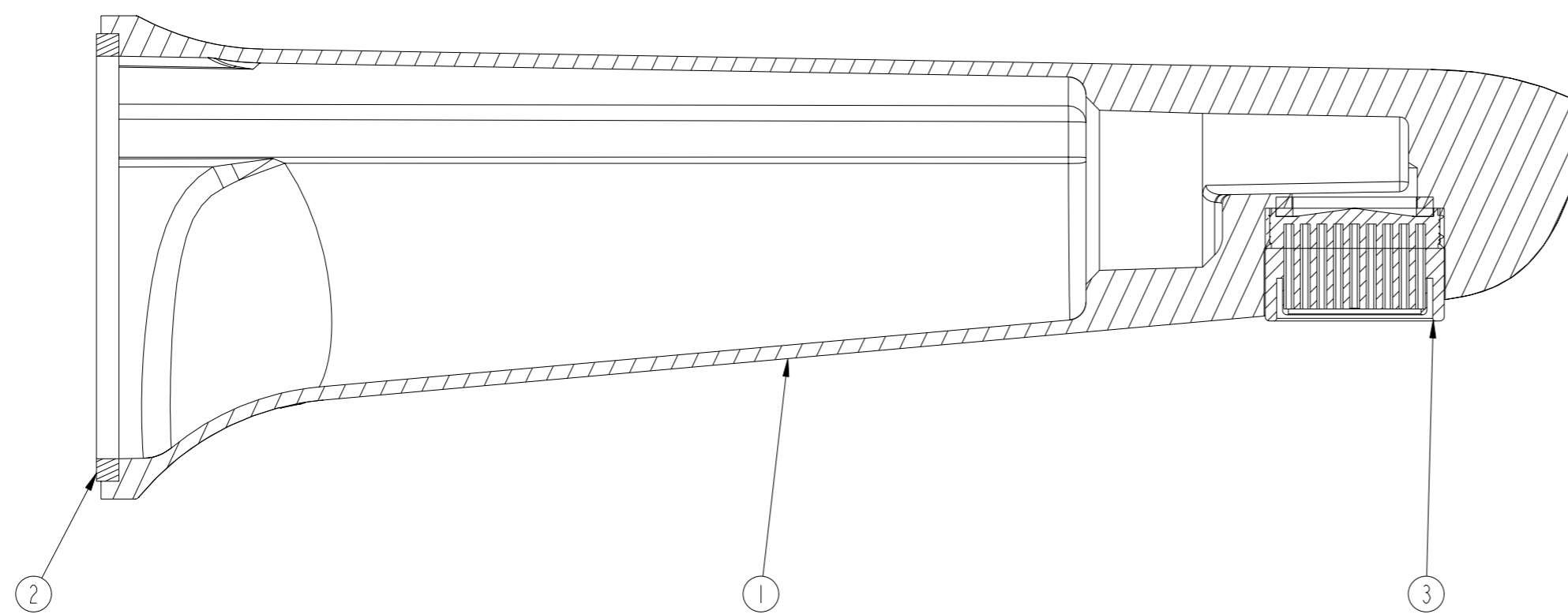
SECTION A-A SCALE 3:2
