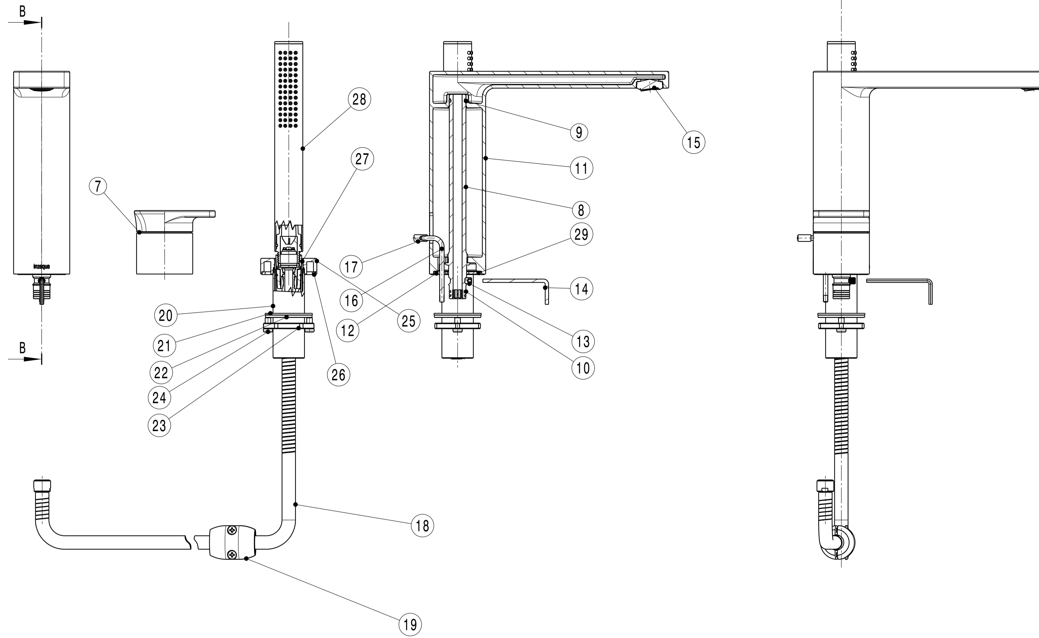
Section view B-B
