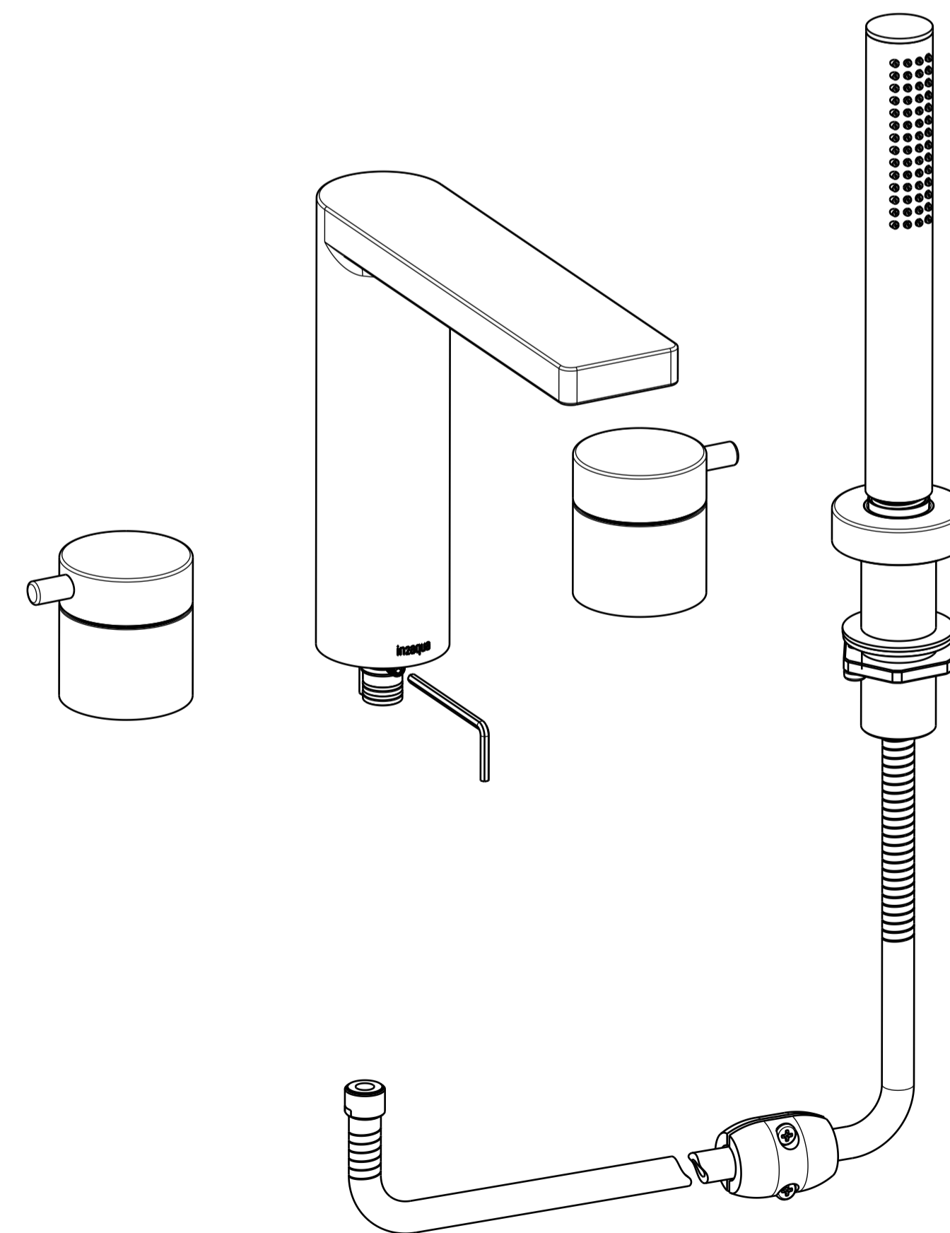
Isometric view
